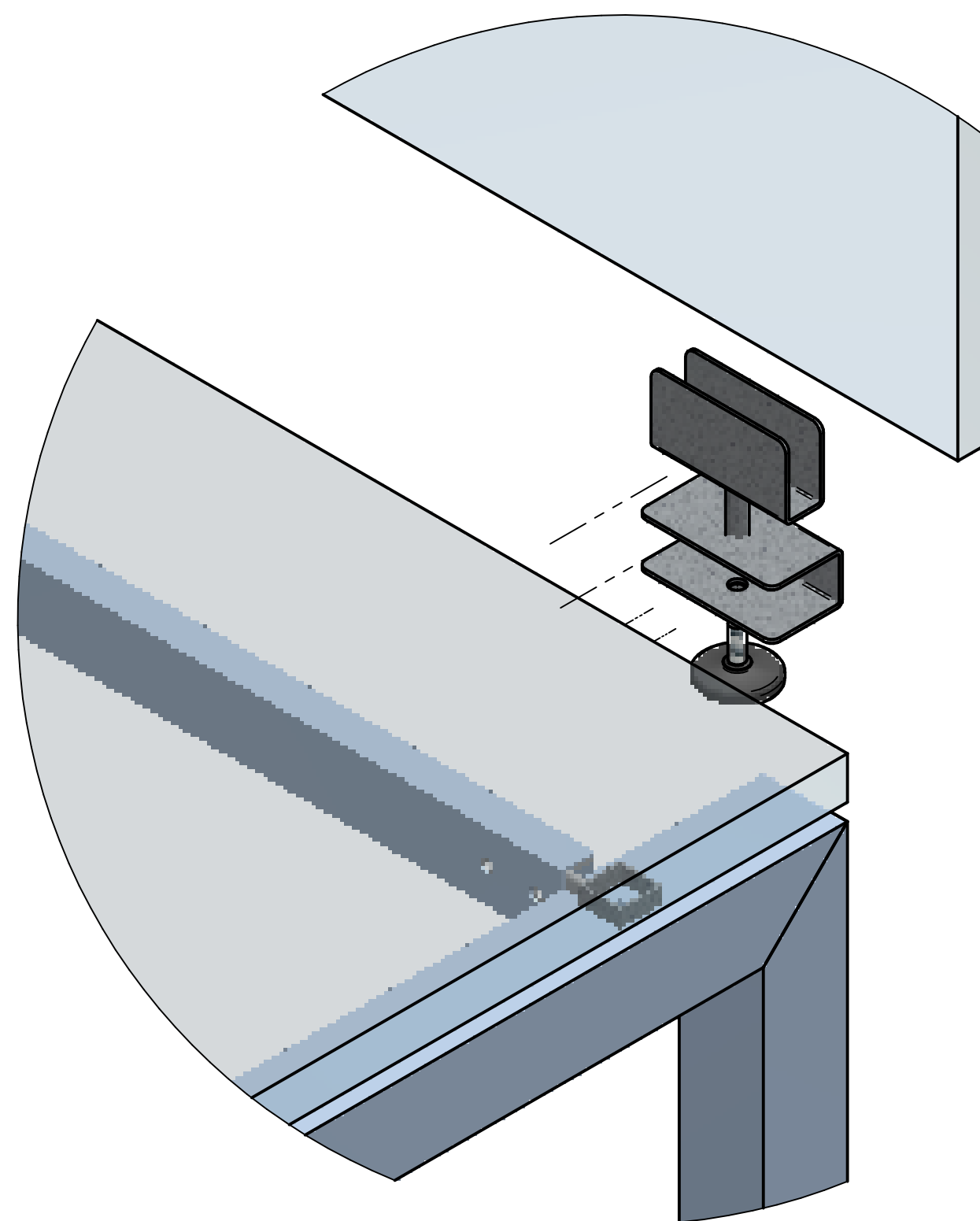
DETAIL B
